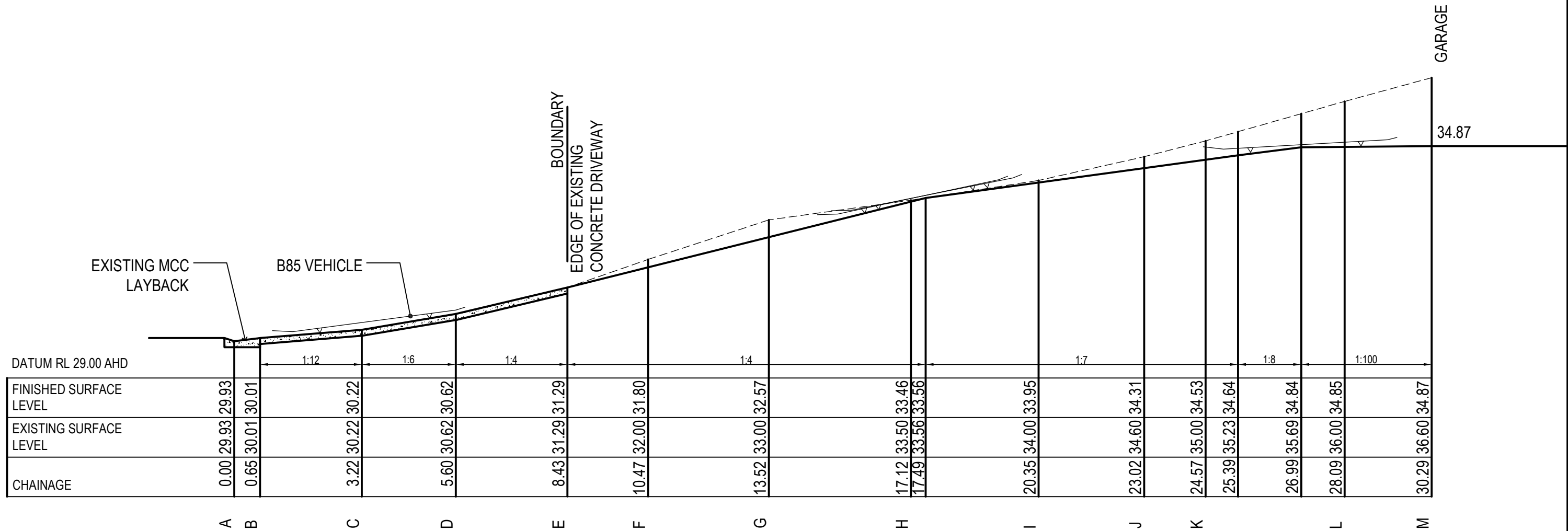
SECTION 1 EASTERN EDGE - CONCRETE DRIVEWAY LONGITUDINAL SECTION 1:100
